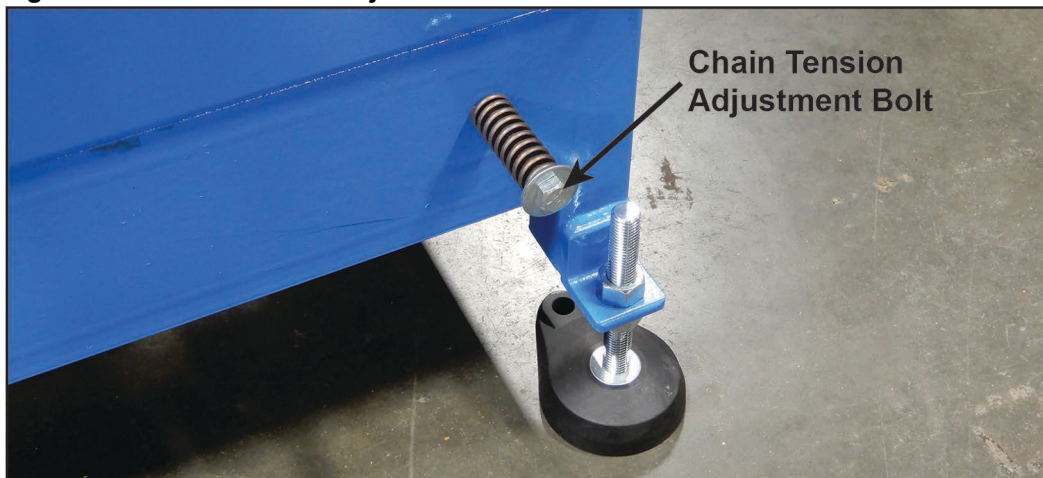
Figure 7-6: Chain Tension Adjustment Bolt
