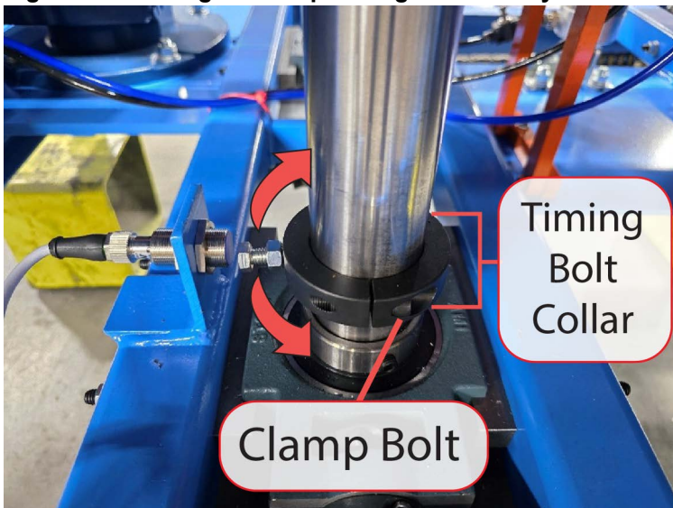
Figure 7-5: Timing Bolt Sequencing to Proximity Sensor
