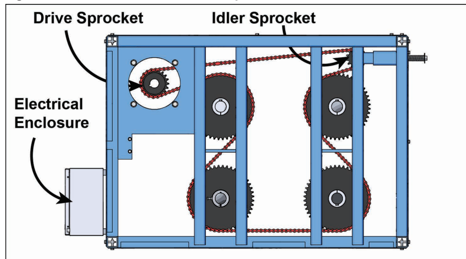
Figure 7-8: Chain Threaded Around Sprockets
