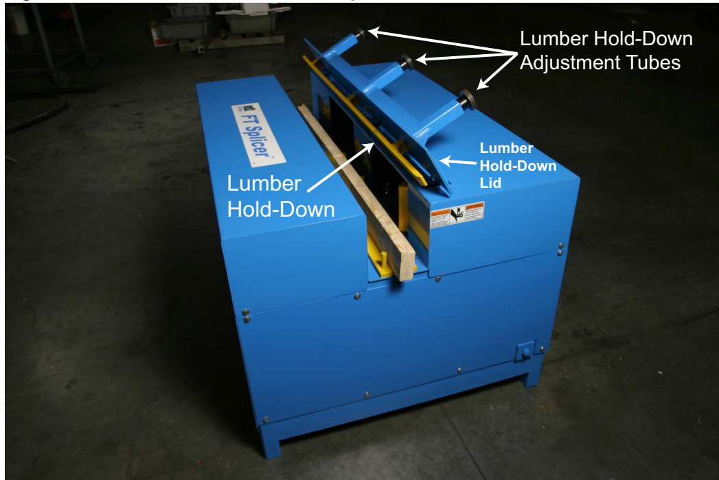
Figure 7-1: Lumber Hold-Down Lid Components
