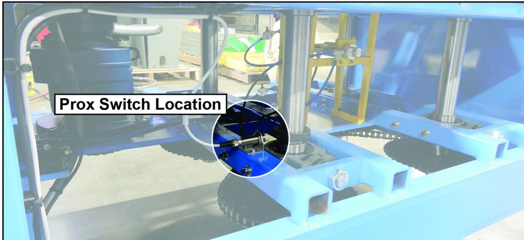
Figure 7-11: Prox Switch Location
