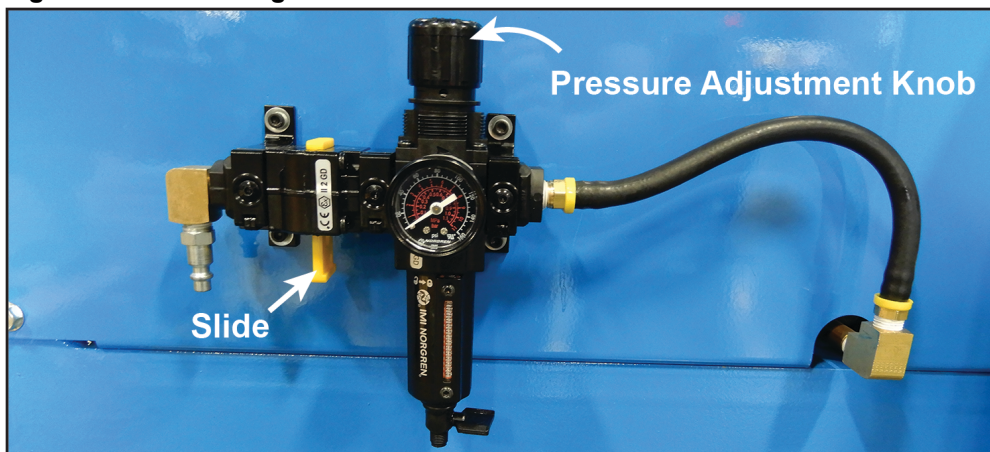
Figure 7-9: Filter / Regulator
