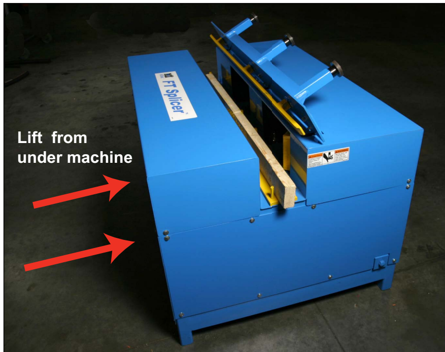
Figure 4-1: Lift Points
