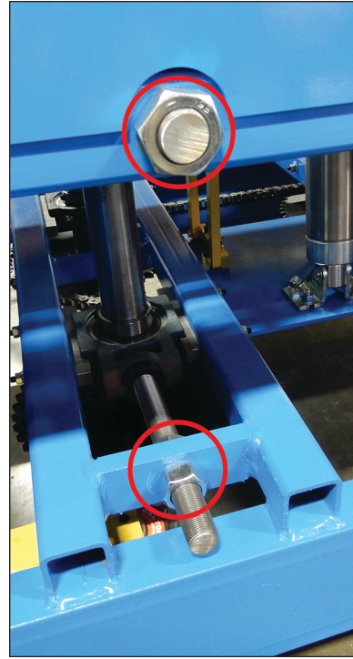
Figure 7-3: Adjustment Nuts
