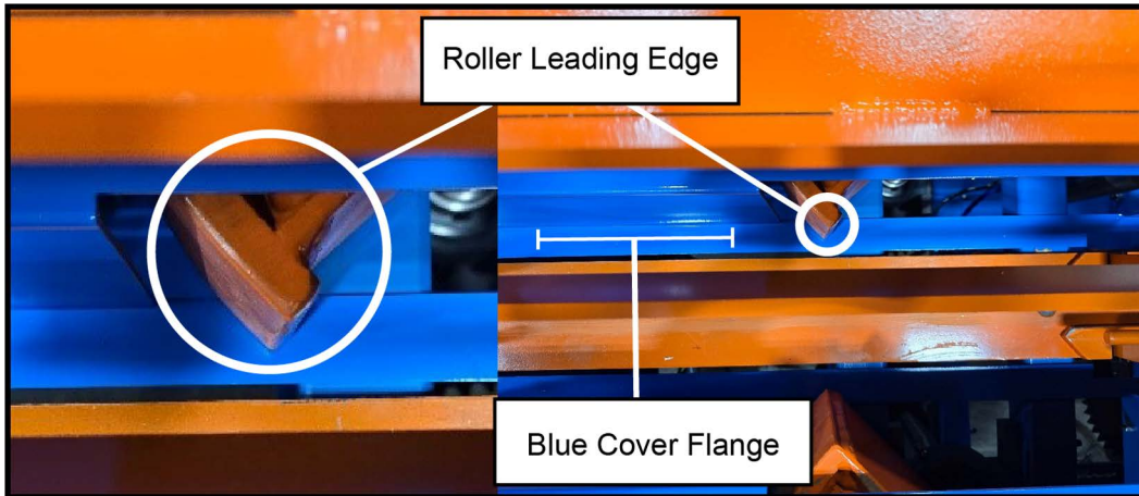
Figure 7-4: Roller Leading Edge Aligned with Blue Cover Flange
